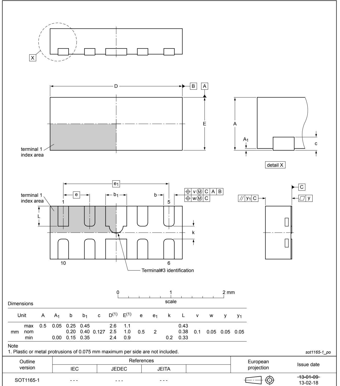
Fig. 1. Package outline DFN2510-10 (SOT1165-1)
